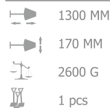
SWG170 ŚWIDER DO GRUNTU 170 MM Ground drill 170 mm
